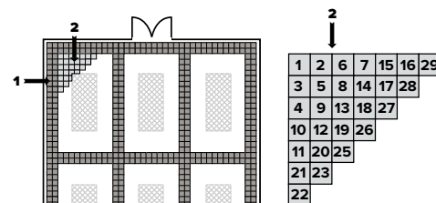
Fig. 6 Installation around fixed objects – laying tiles
