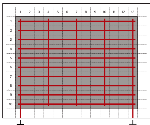
Fig. 3 Installation of grounders tape.
