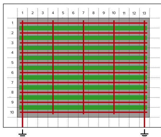
Fig. 4 Installation of the system with fixing tape.
