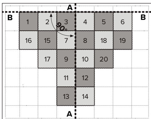
Fig. 3 Installation of grounders tape.
